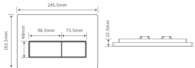
SQUARE FLUSHPLATE
